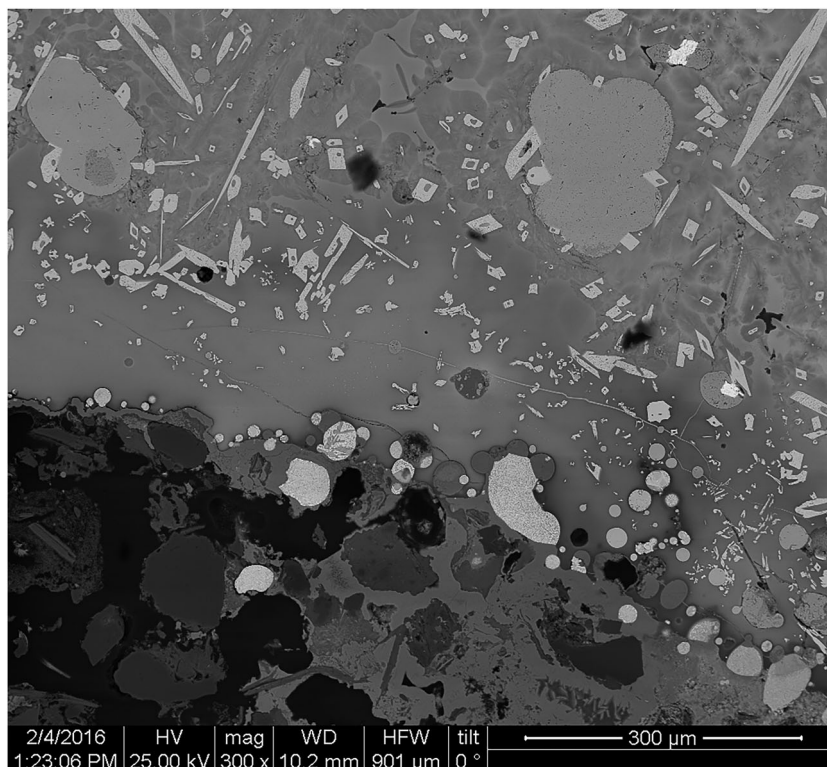
Figure 8. SEM/EDS photomicrograph of crucible slag (THB07aE). Globular and spheroid Cu–Sn–Pb inclusions, bronze kidney-shaped inclusion, elongated lamellae and rhomboid crystals of tin oxide with filled crystals cores, typical evidence for newly formed tin oxide, and glassy matrix (dark grey).
