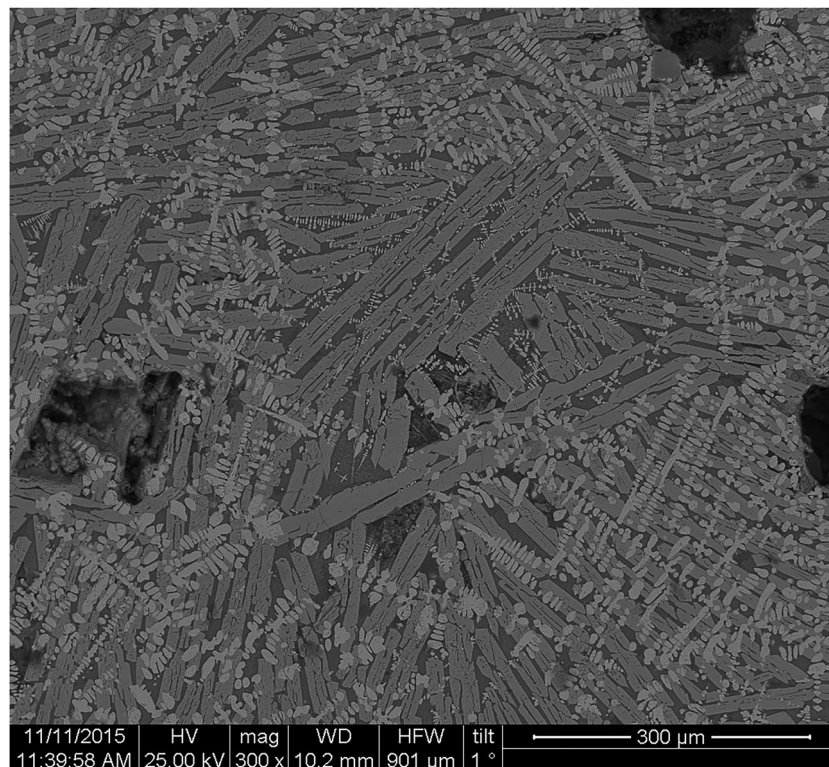
Figure 5. SEM/EDS photomicrograph of iron slag (TBH07aA). The microstructure consists of fayalitic laths (mid grey), wüstite dendrites (light grey) and a glassy matrix (dark grey).
