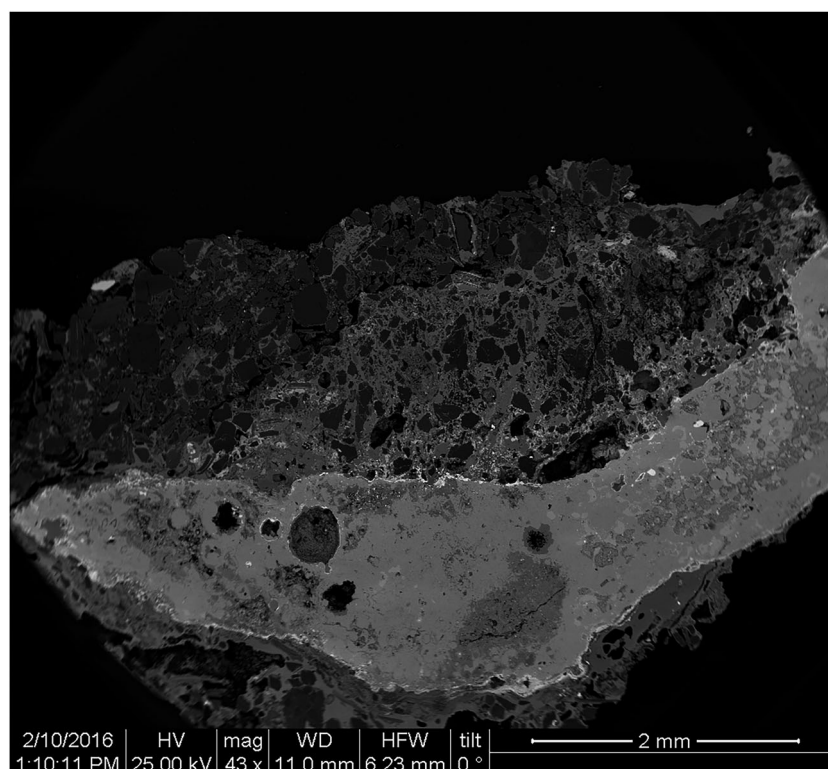
Figure 11. SEM/EDS photomicrograph of crucible THB09D. Three zones: peripheral ceramic (dark grey-upper part), porous interface (mid grey), slag zone (light grey-lower part).
