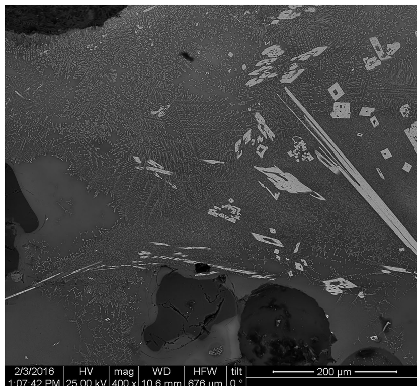
Figure 9. SEM/EDS photomicrograph of crucible slag (THB11 g). Lamellar and rhomboid, newly formed tin oxide crystals with filled cores (light grey), glassy matrix (dark grey).
