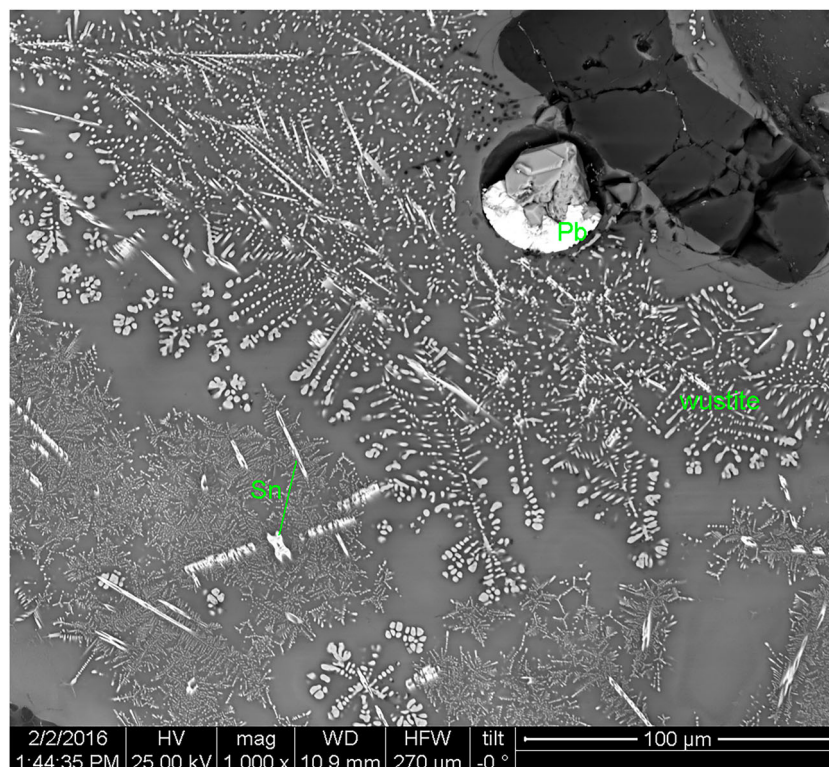
Figure 7. SEM/EDS photomicrograph of crucible slag (THB11 g) showing dendritic phases of Cu-Sn-Pb composition (white), elongated lamellae of tin oxide, a Pb-rich inclusion and glassy matrix.
