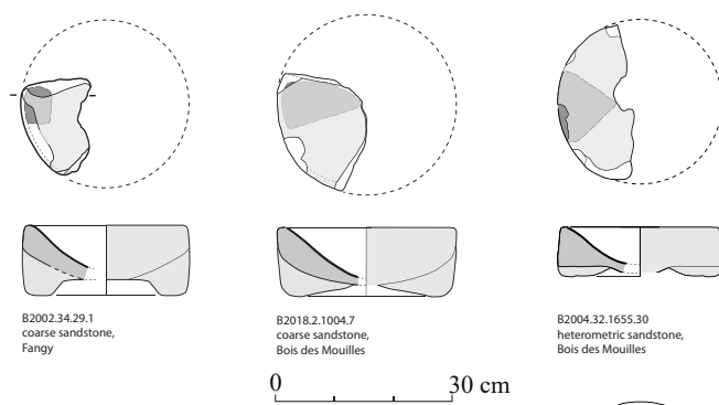
3 variants of tripod mortars
