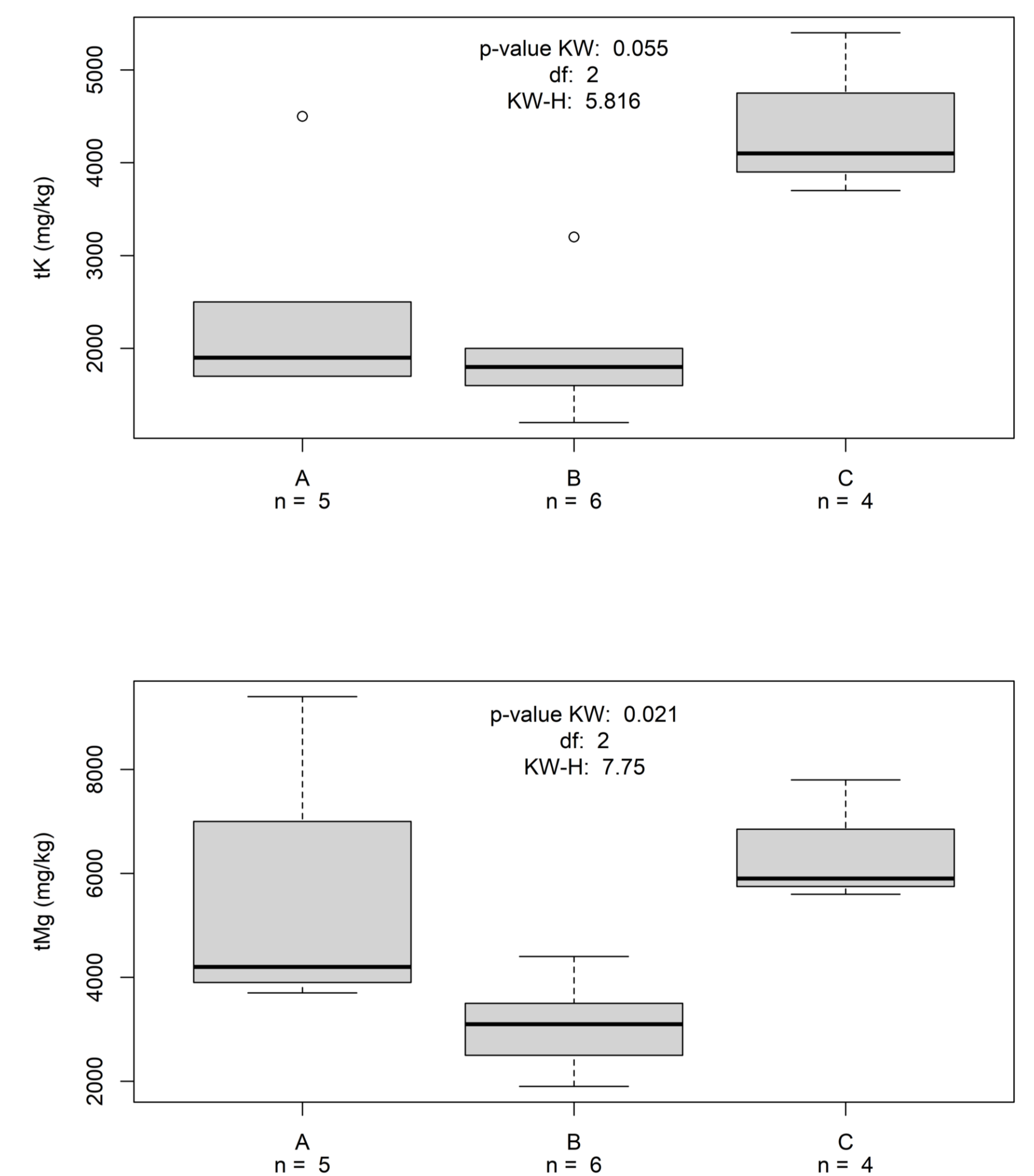
Figure 4. Chemical analysis determined: dark layer (A), sandy layer (B) is often without the human influence (depleted), geological substrate of alluvial plain (C).
