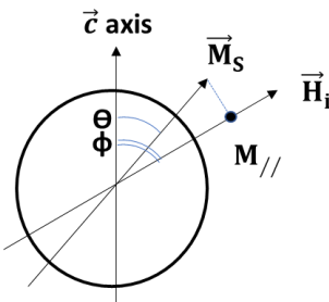
Fig. A1 . Spherical particle with uniaxial magnetocrystalline anisotropy.
